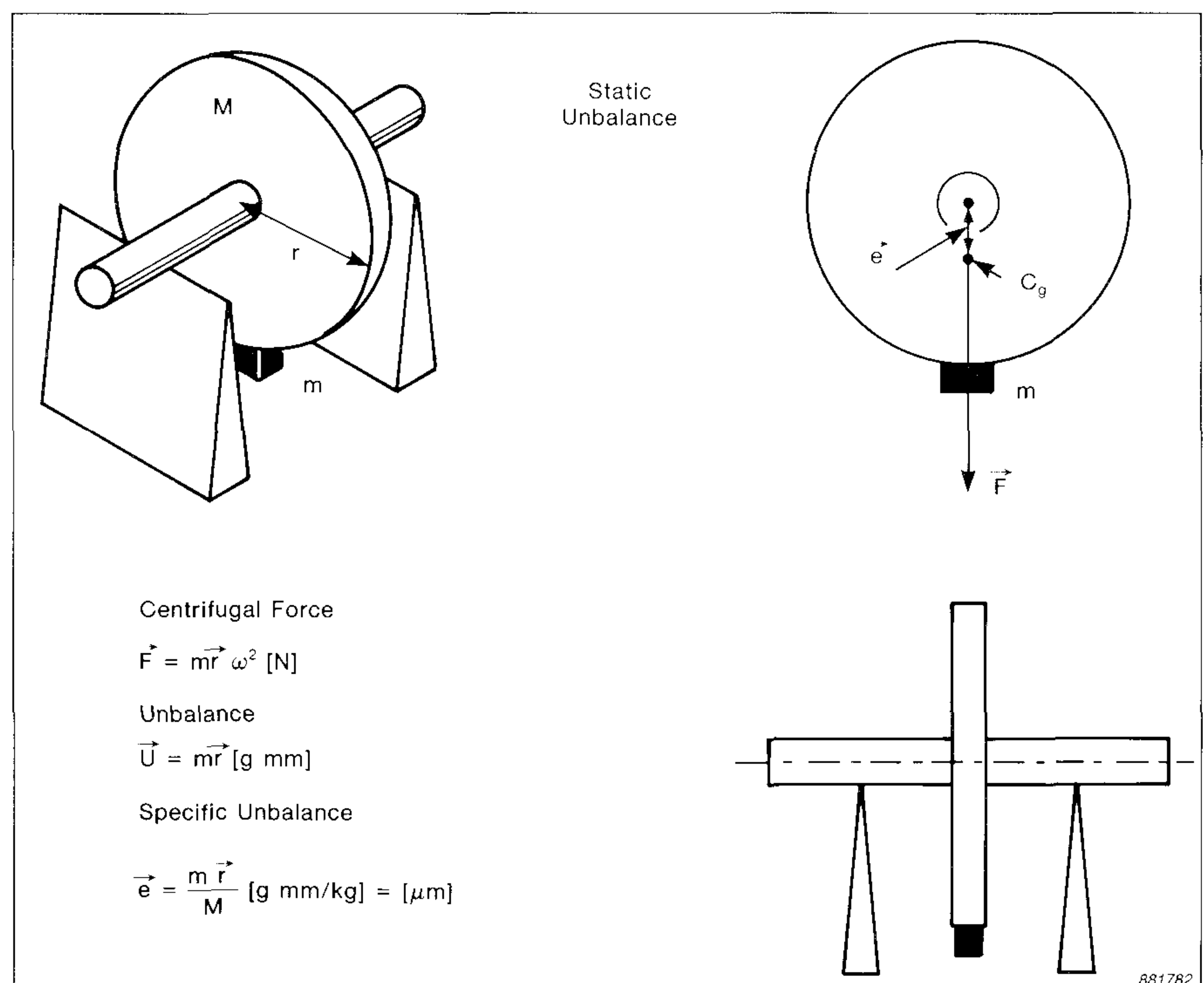
Fig. 1. Static unbalance
