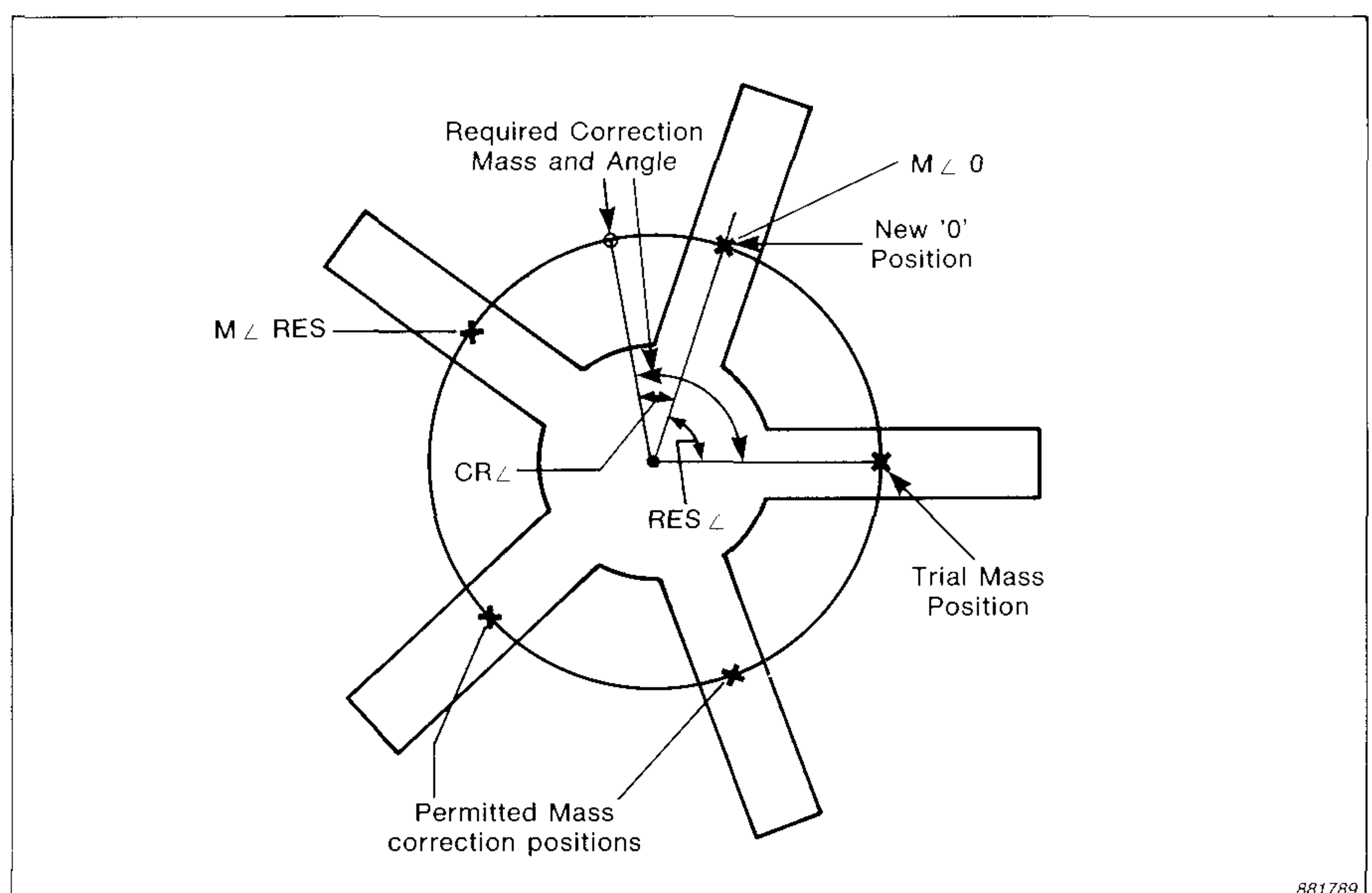
Fig. 18. Dividing a correction mass into two components for mounting on a five-blade fan
