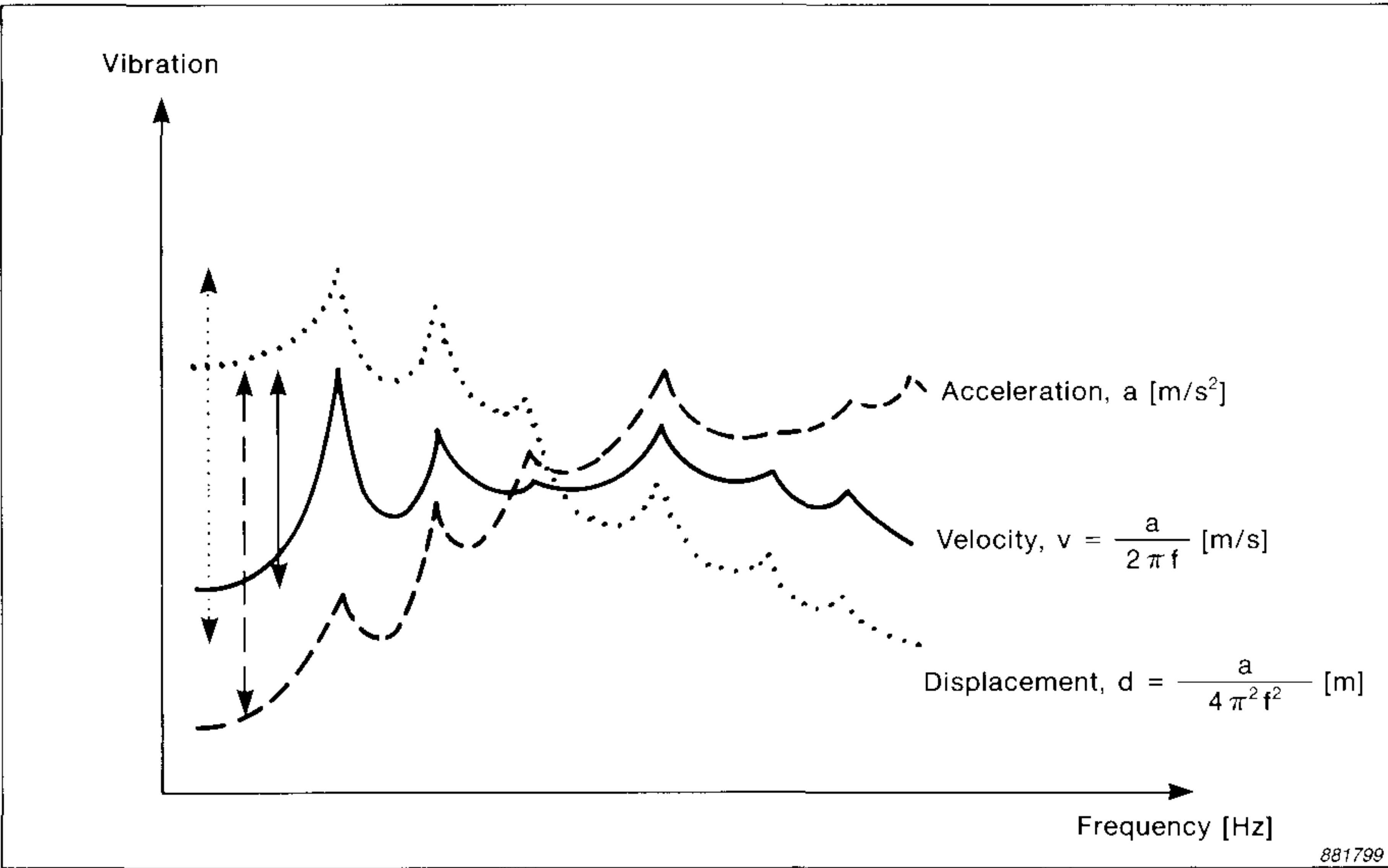
Fig. 7. Frequency spectra produced using three different measurement parameters: acceleration, velocity and displacement. The signal range for each parameter is shown
