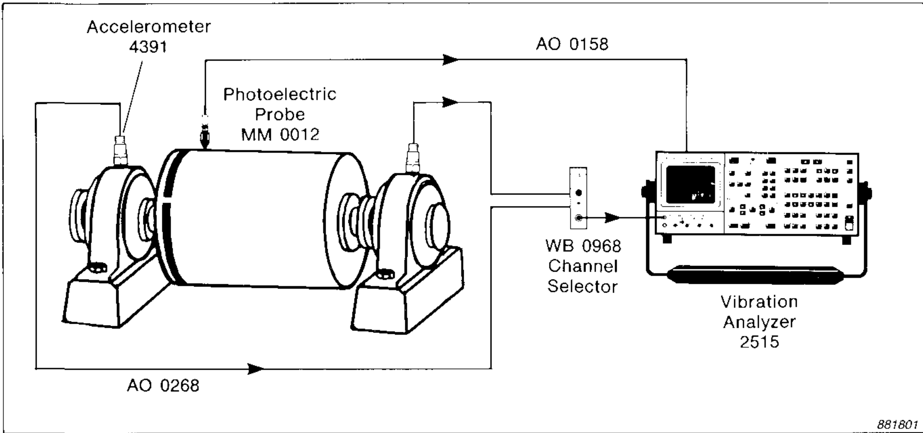
Fig. 31. Instrument set-up for Example Two
