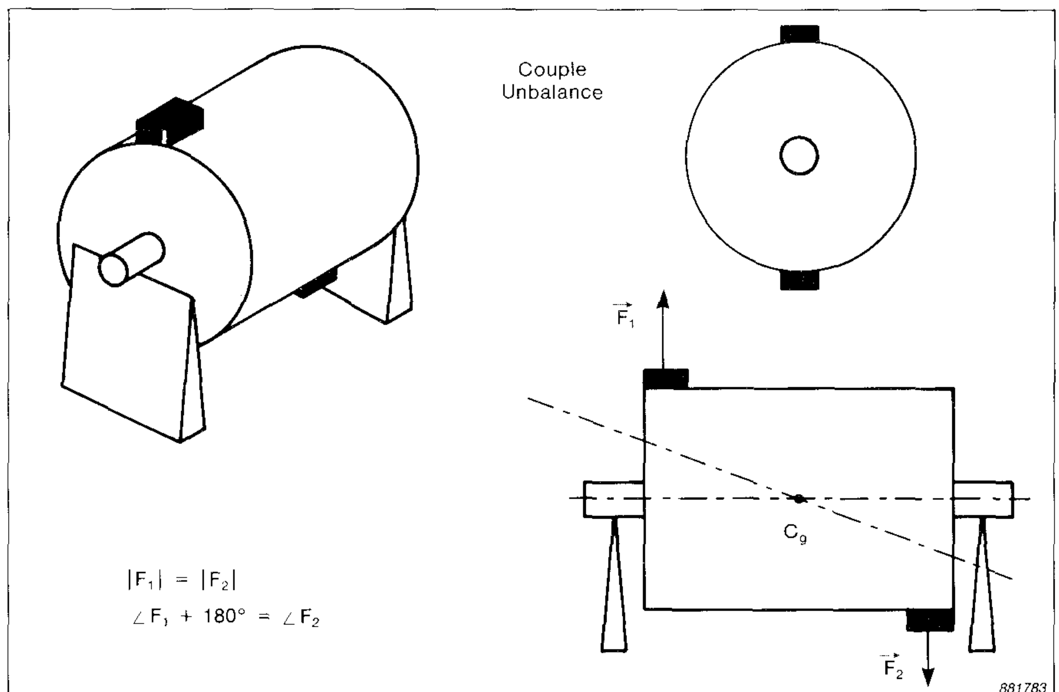
Fig. 2. Couple unbalance
