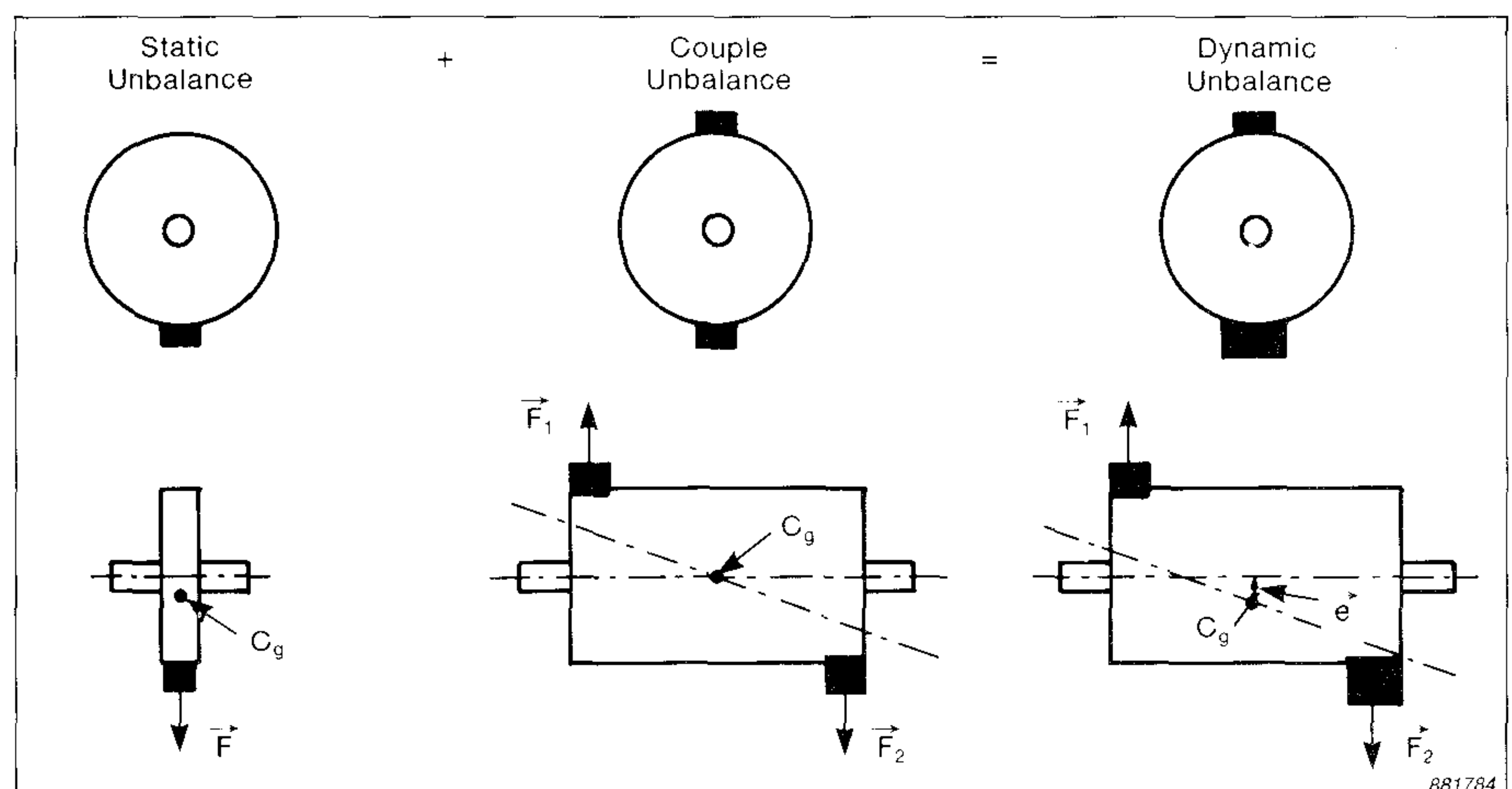
Fig. 4. Dynamic unbalance
