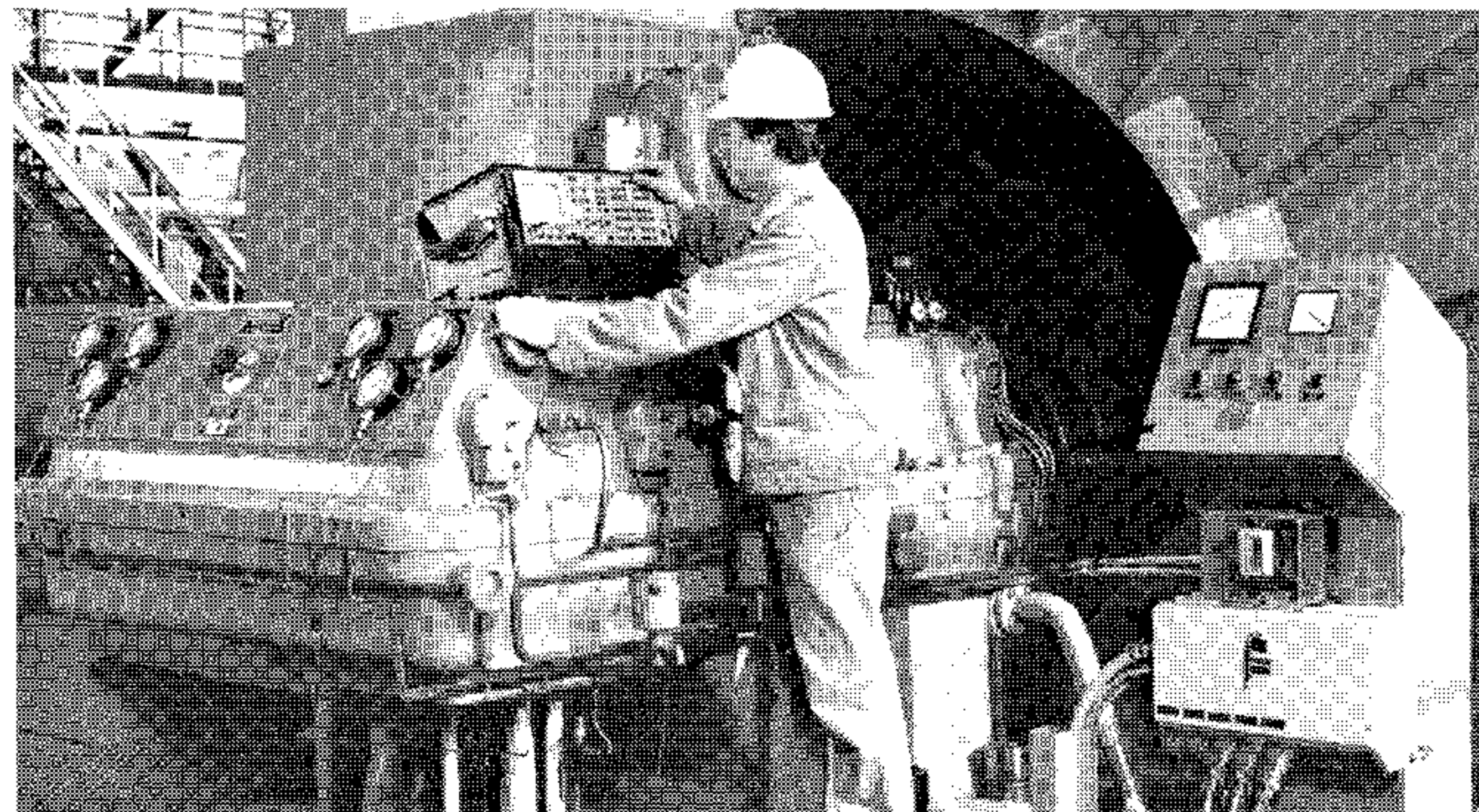
Fig. 19. To the left, the Vibration Analyzer Type 2515. To the right, balancing a 275 MW turbo-generator set at Kyndbyværket power station
